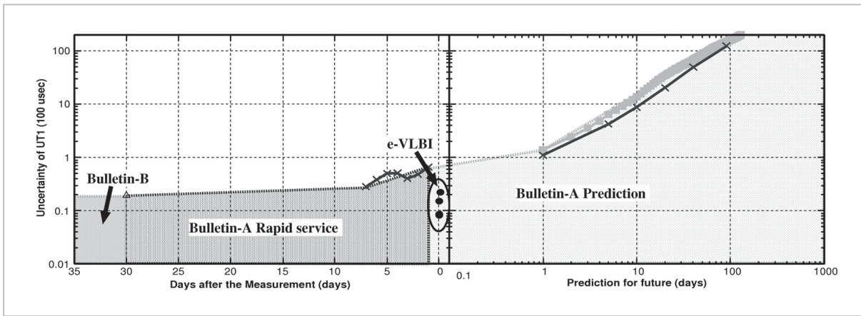
Fig.3 Uncertainty of UT1 from the IERS bulletins
