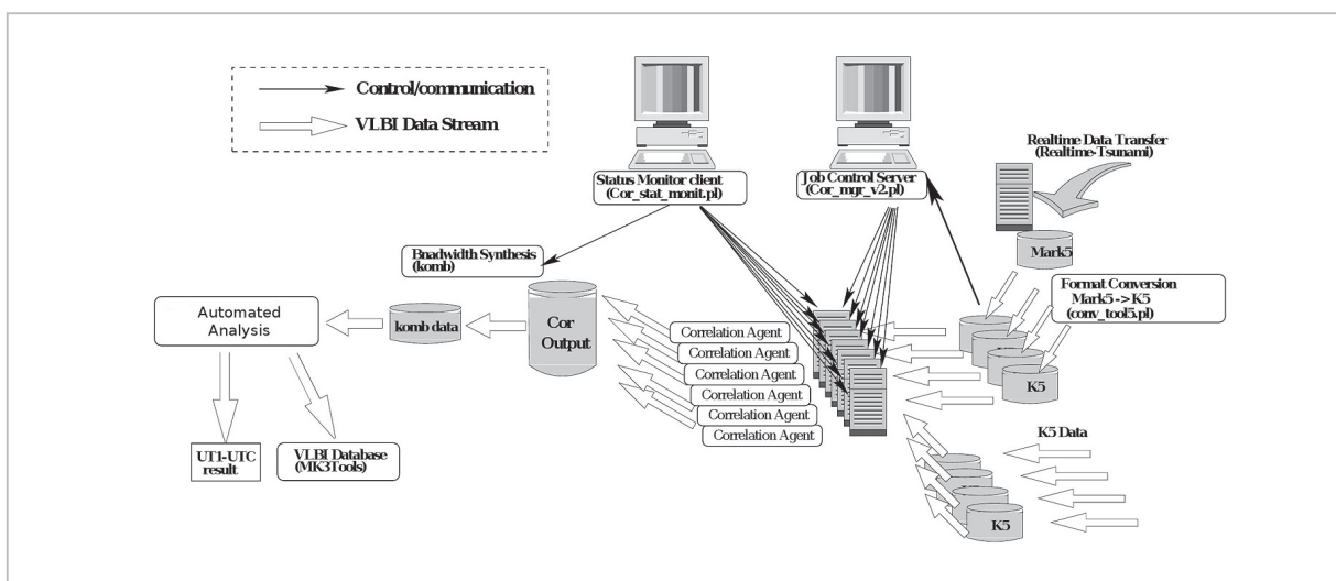
Fig.4 Automatic data processing which takes advantage of a distributed computing environment
